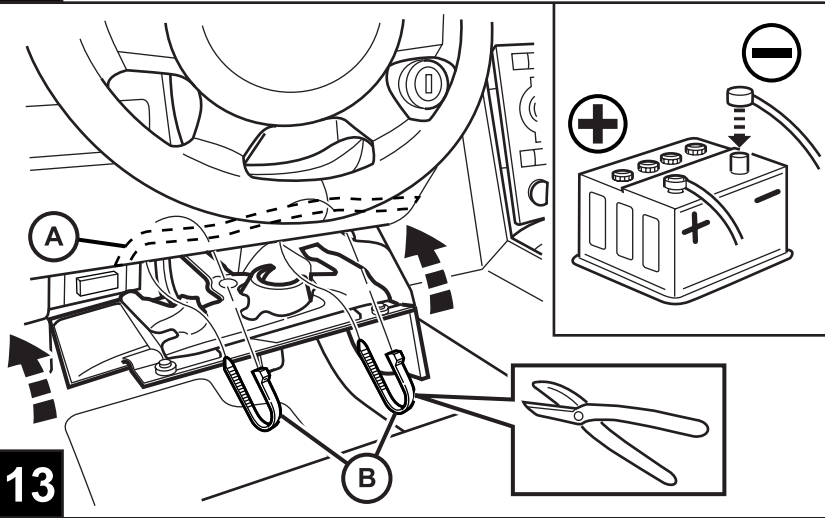
FACTORY INSTALLED 7-WAY TRAILER TOW INSTALLATION EN USINE INSTALACION DE FÁBRICA
